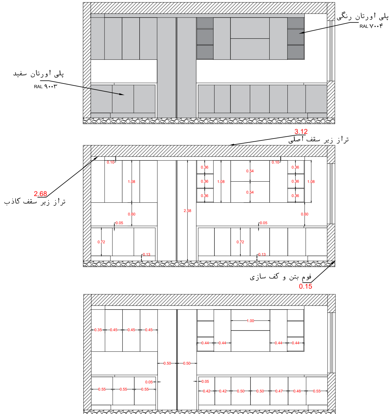
Section- F-F
