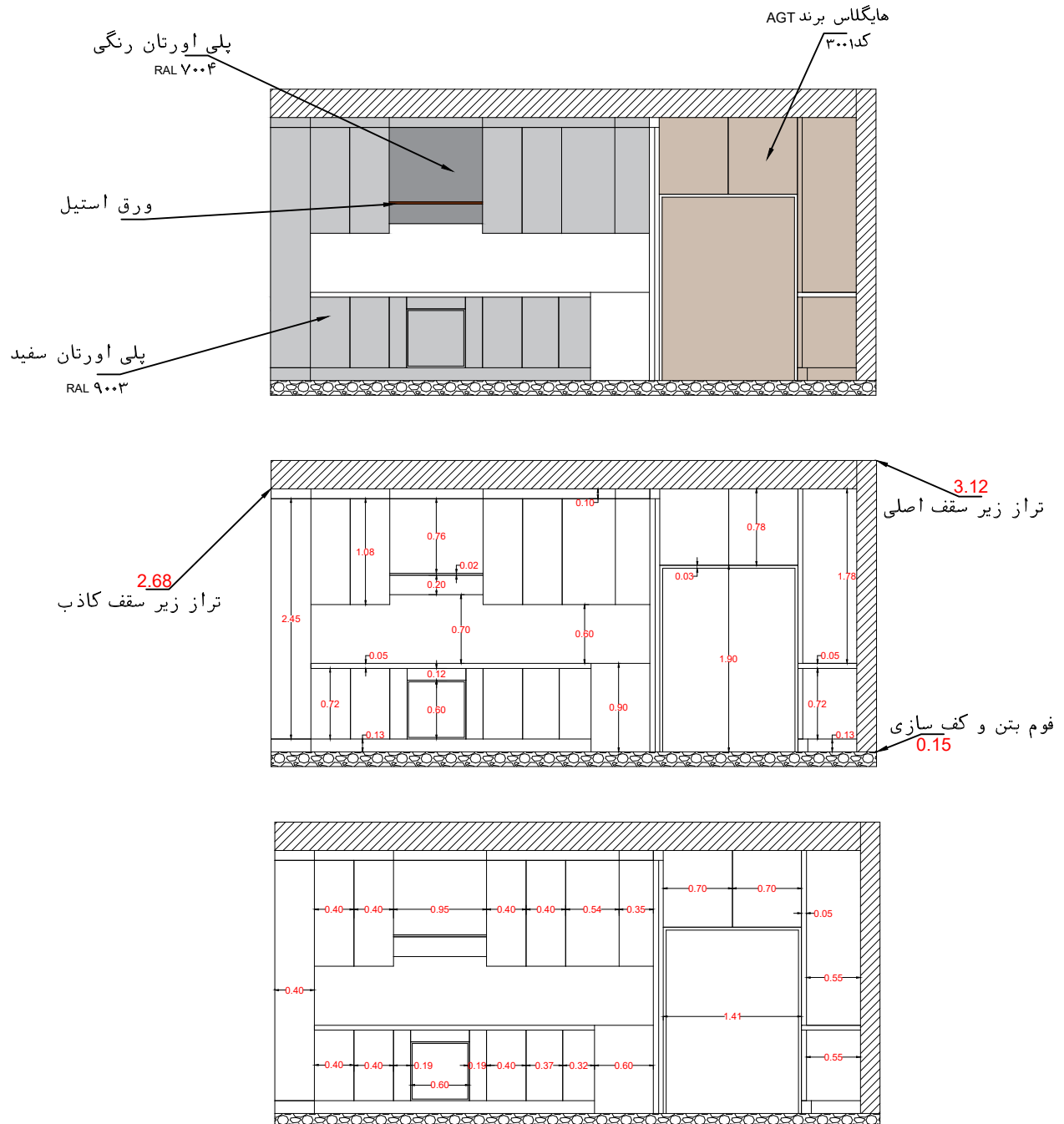
Section- E-E
